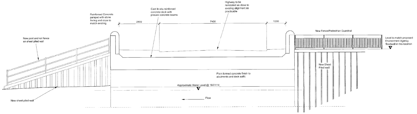
Sectional Elevation B-B (View on Southern Abutment)
